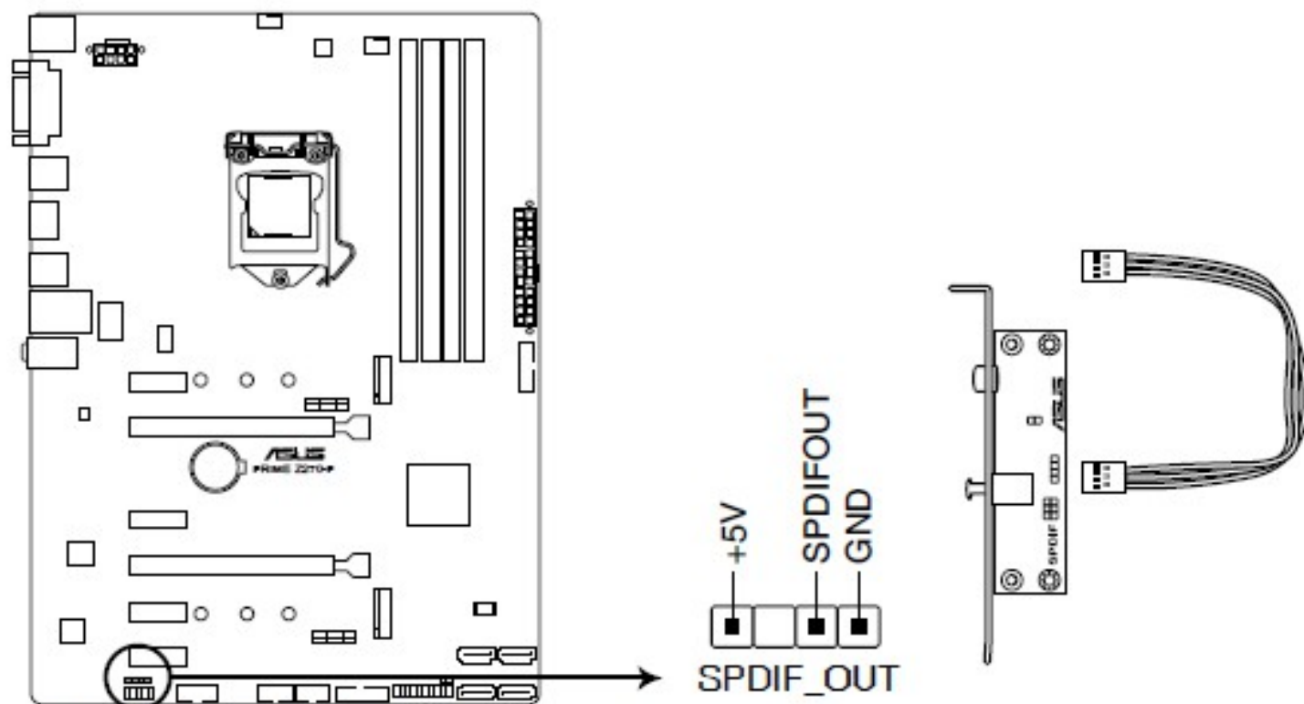
PRIME Z270-P Digital audio connector
