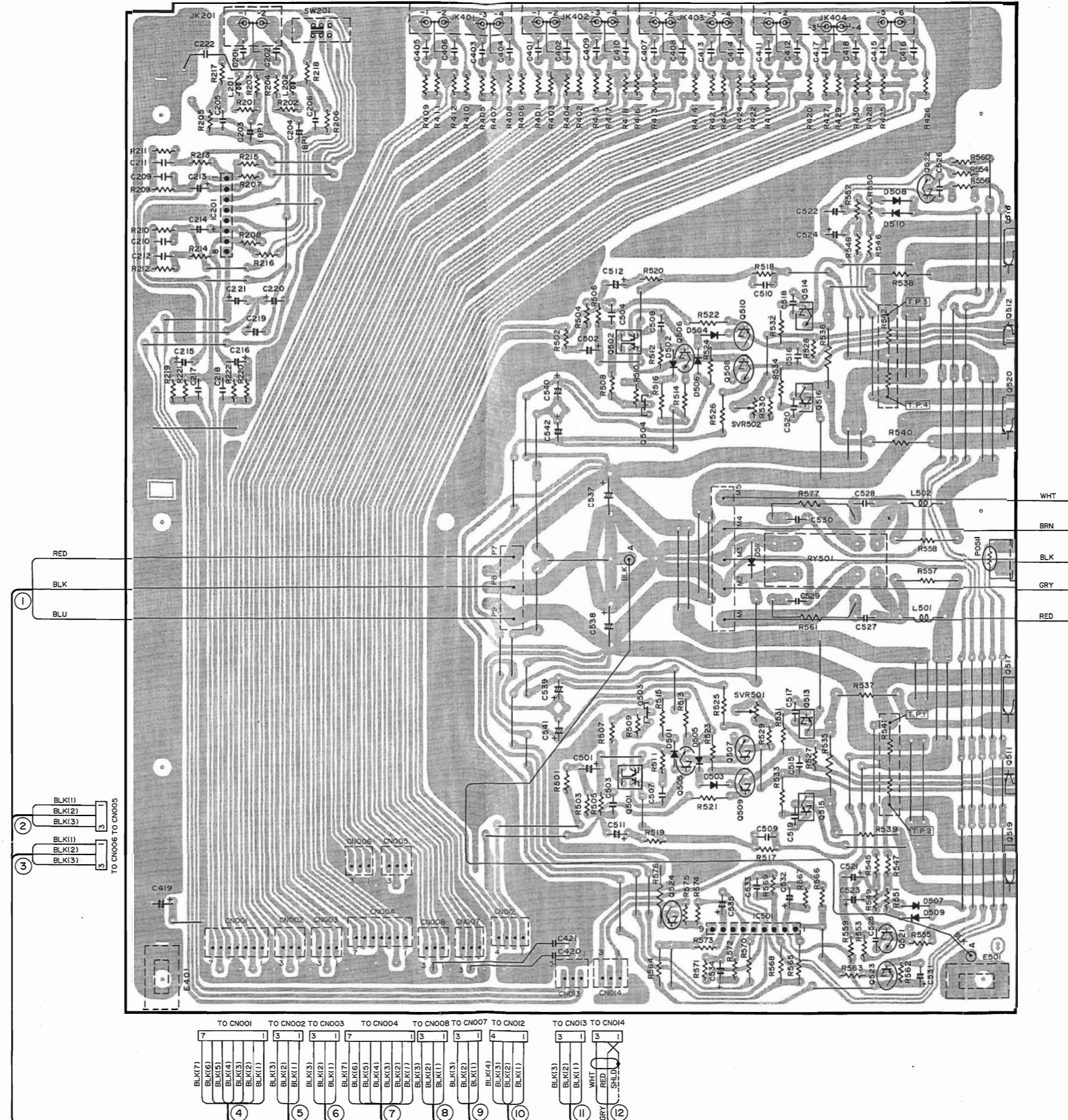
MAIN P.C. BOARD
