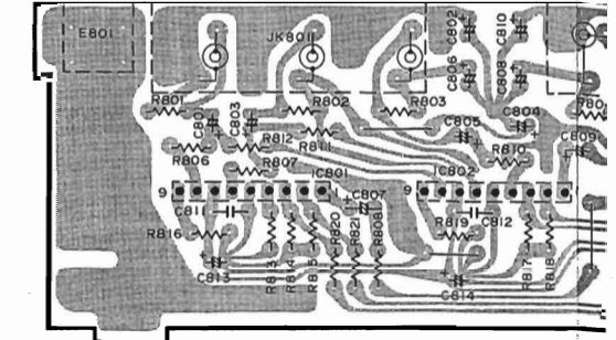
VIDEO P.C. BOARD (★)
