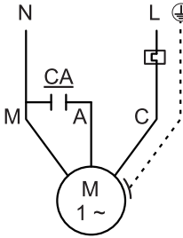
Single phase with capacitor connection demonstration
