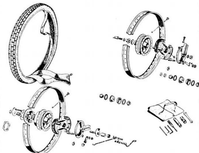
T. VIII - Front and rear wheel Page 30
