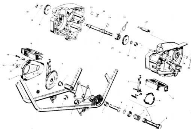
T. X - Frame - Vehicle with Pedals Page 38
