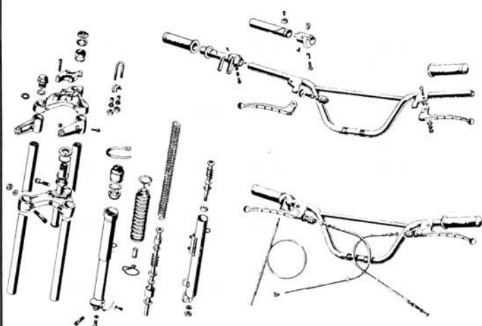
T. VII - Front suspension - Handlebars and controls Page 26
