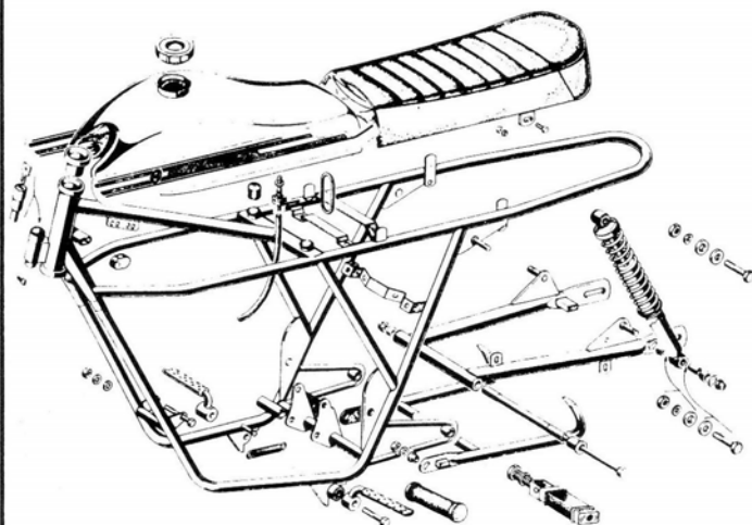
T. V - Chassis - Rear suspension - Fuel tank - Saddle Page 20
