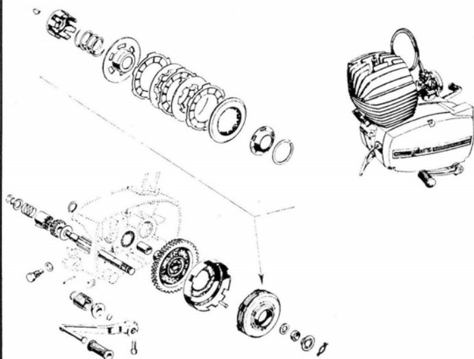
T. III - Cylinder and piston assy. - Crankcase and covers - Clutch control Page 12
