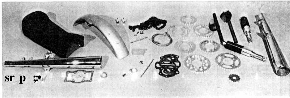
This is the basic kit for notable improvement in performance and includes not only racing seat and lobed rear fender but also stiffer front fork springs and rear suspension units along with a full set of sprockets. YB72 8800A
