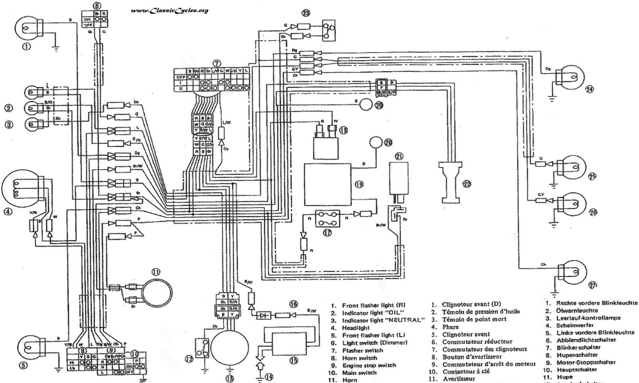
Yamaha LB50 LB80 Chappy Electrical Wiring Diagram Schematics
