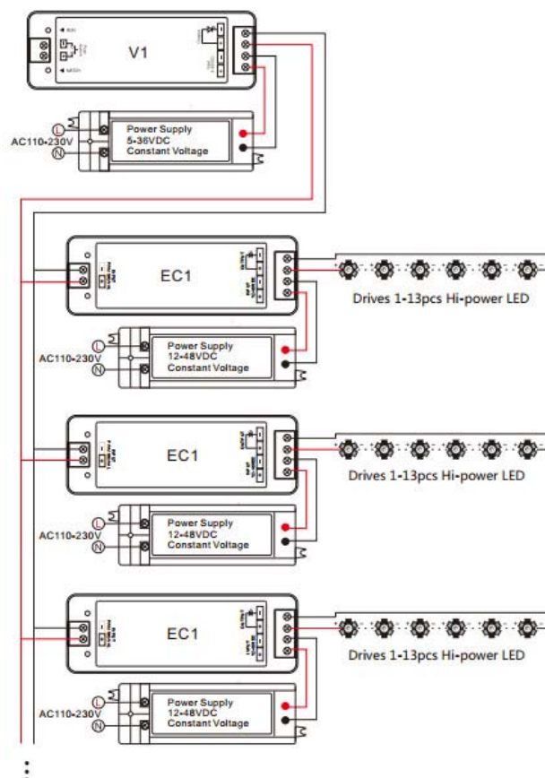
One V1 parallel connect with multiple EC1
