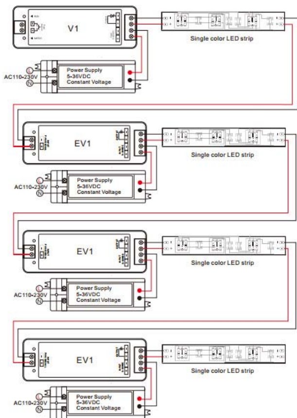
One V1 series connect with multiple EV1
