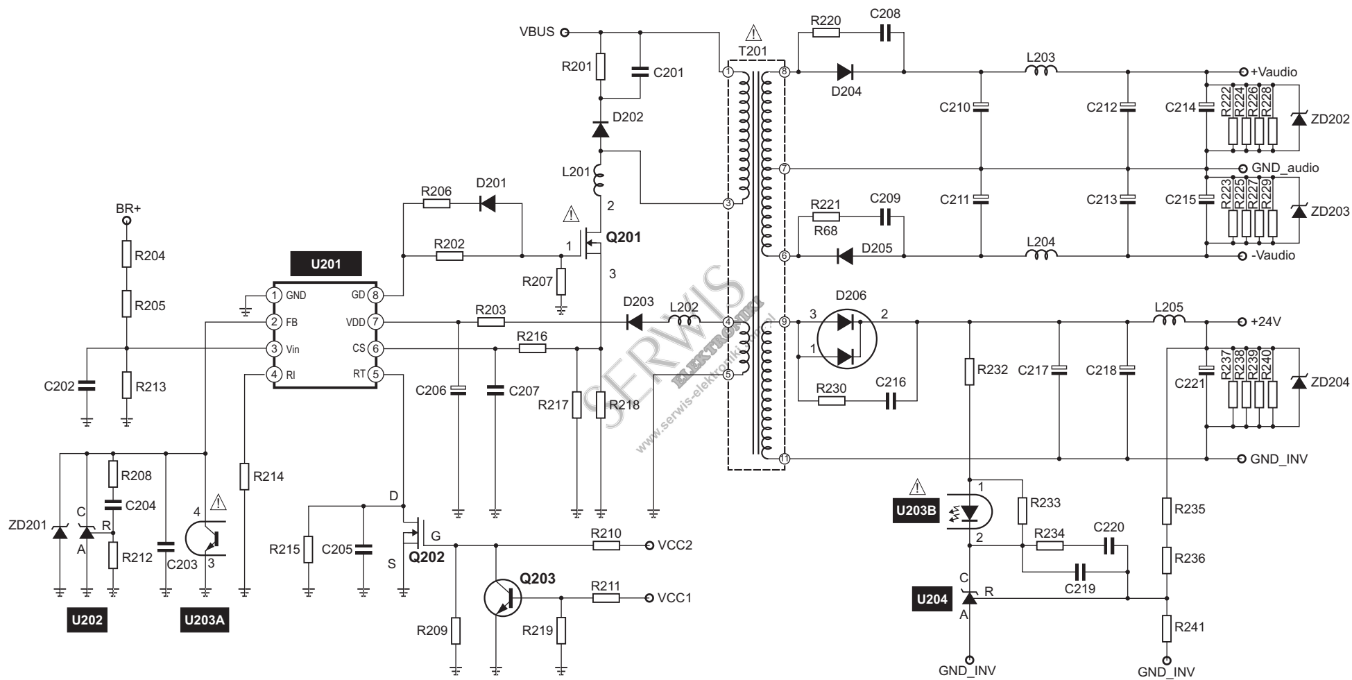
DAC-12M058 AF-S-R0C9X09.SCH
