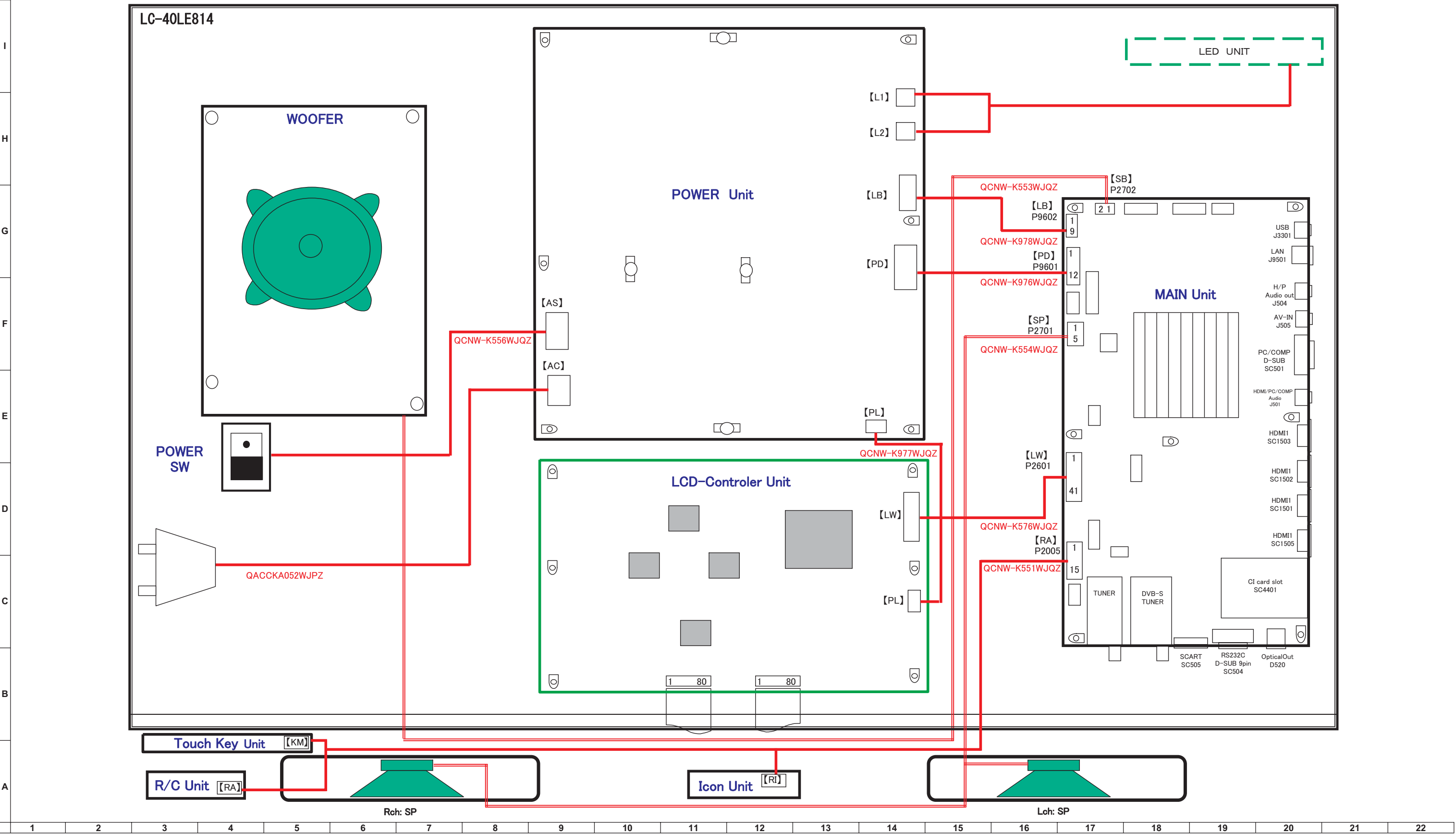
[1] OVERALL WIRING DIAGRAM (LC-40LE814E/RU)
