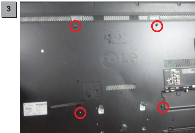
Disassemble 4 VESA screws.
