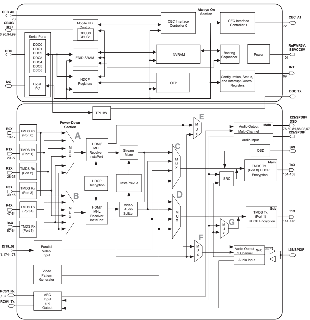
IC202: SI9573CTUC HDMI port processors
