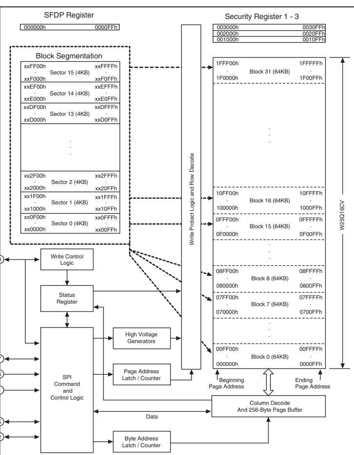
IC201: W25Q16CVSSIG 3 V 16 M-bit serial flash memory with dual and quad SPI
