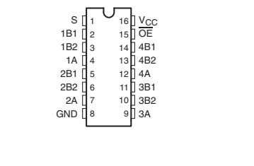
IC204: TC7VH04FU 4-bit 1-of-2 multiplexer/demultiplexer
