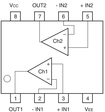
IC23-25, 27: BA4560F-E2 Low noise dual operational amplifier
