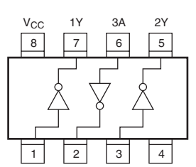
IC203: TC7VH04FU Triple inverter
