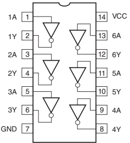
IC22: TC74VHC04FT Hex inverters
