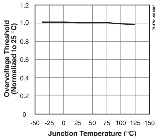
Figure 42. Overvoltage Threshold vs. Temperature.
