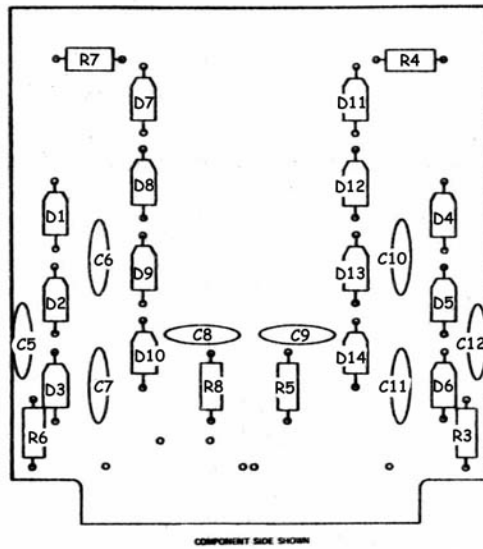
Fig. 11 E-9 Circuit Board.
