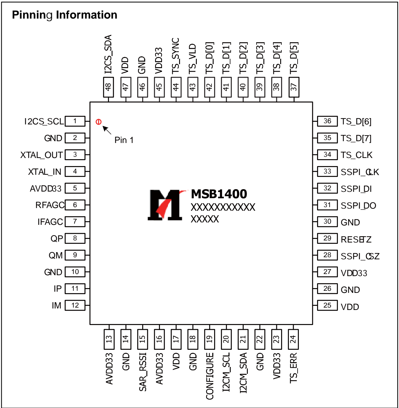
Figure 8-2 Internal pin configuration
