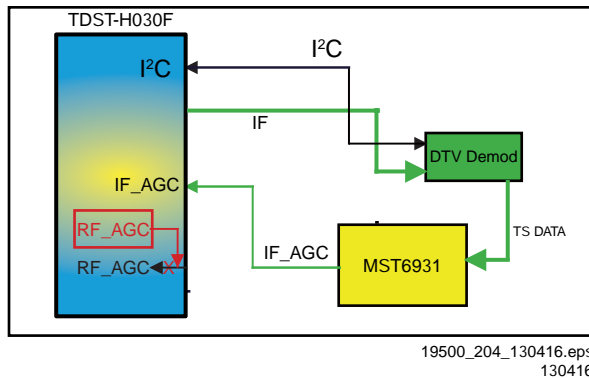
Figure 7-5 Front-End DVB-T2 DTV block diagram
