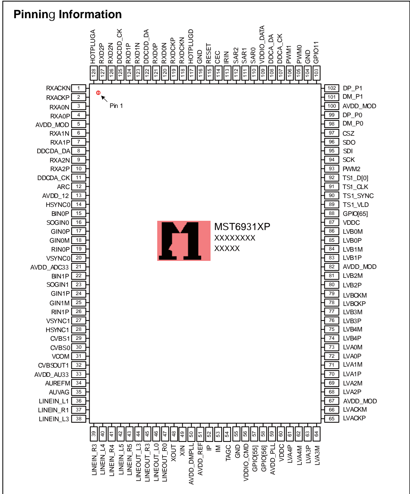
Figure 8-1 Internal pin configuration
