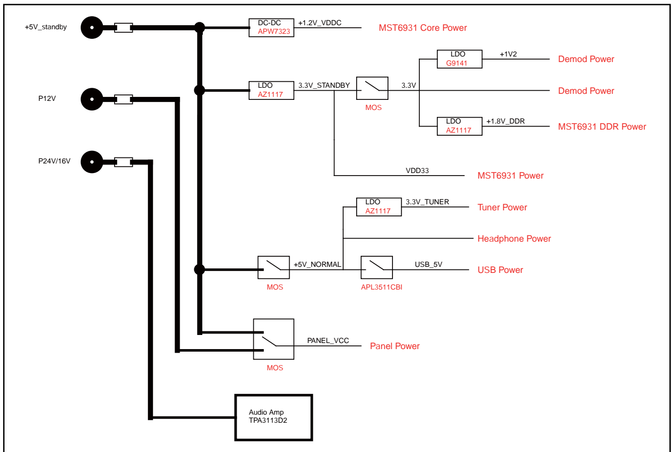
Figure 7-3 DC/DC converters
