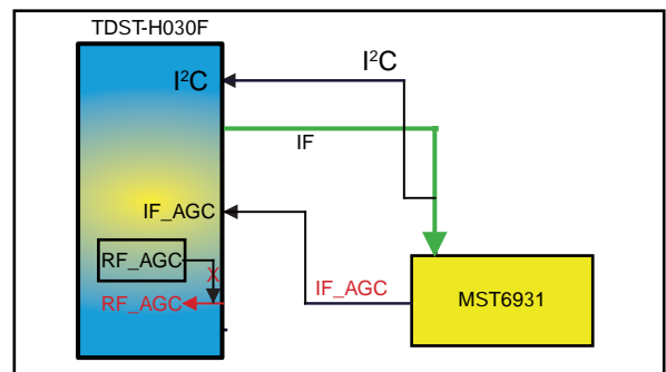
Figure 7-4 Front-End DVB-T/C DTV block diagram
