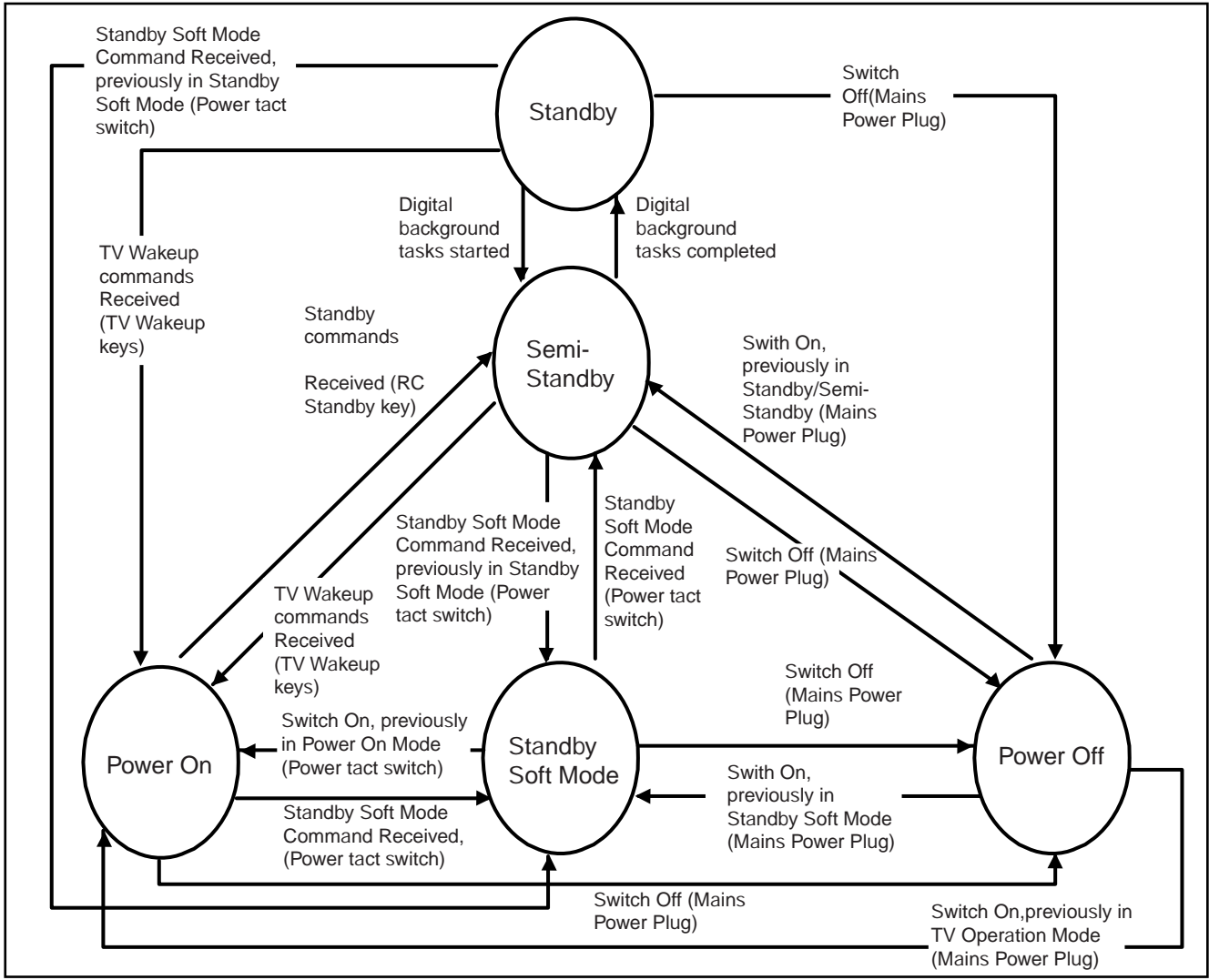
Figure 5-1 Stepwise Start-up
