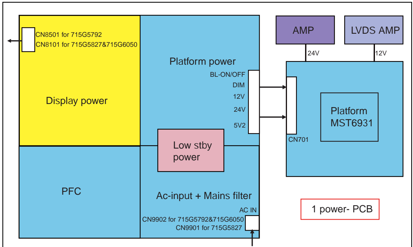
Figure 7-2 Power Architecture
