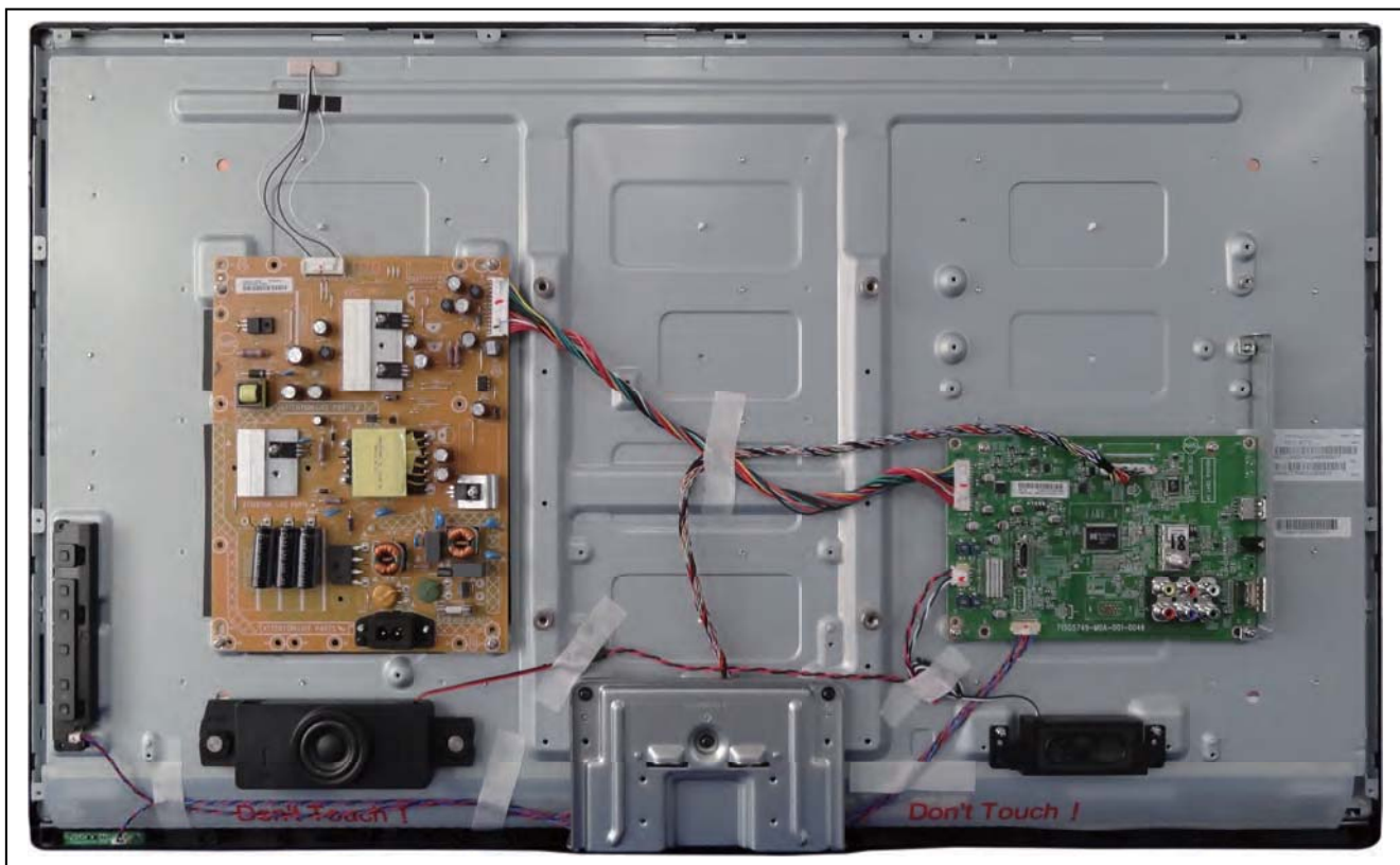
Figure 4-2 Cable dressing (39" 3000 series)
