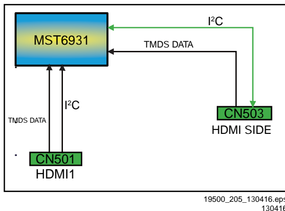
Figure 7-6 HDMI input configuration
