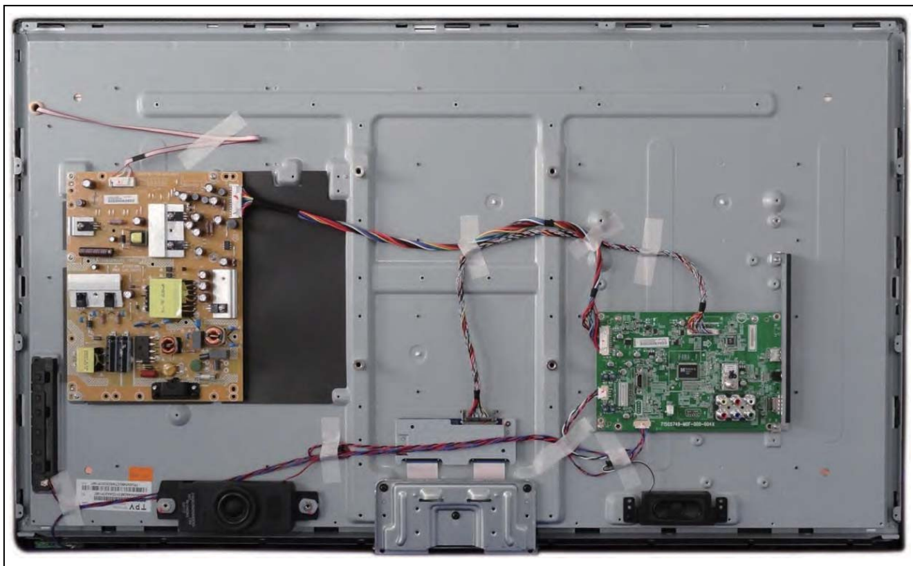
Figure 4-3 Cable dressing (42"-46" 3000 series)
