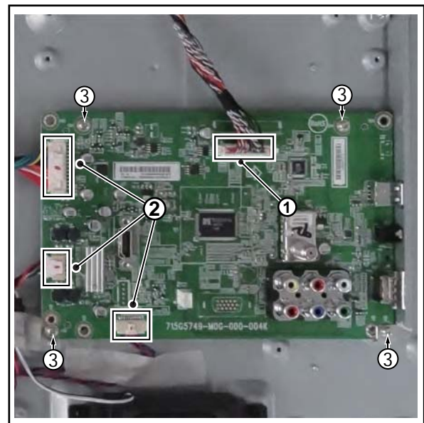
Figure 4-5 SSB removal
